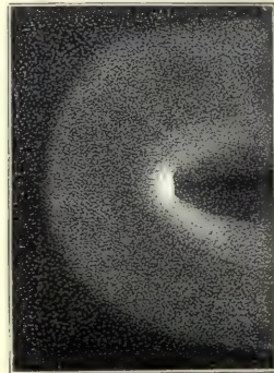
October 6. (Pepe.)
